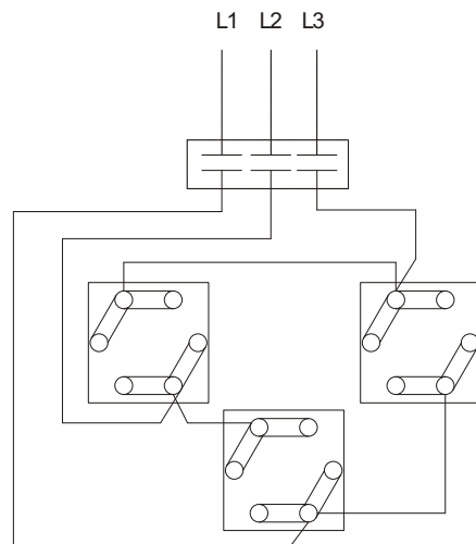
THREE PHASE 25 KW/30 KW (440-480V.)
